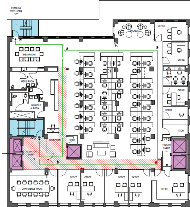
12 th FLOOR
